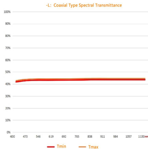
SMT11IR4W65C-L
