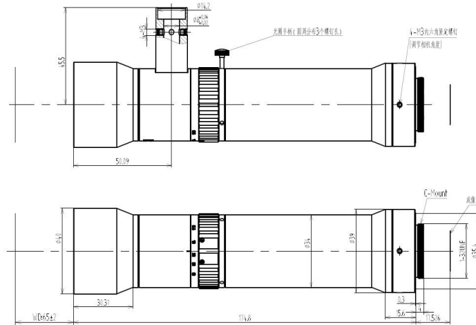
SMT11IR4W65C-L
